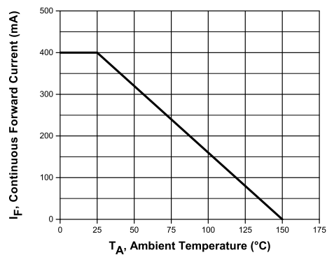
Current Derating
