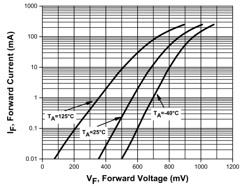
Forward Voltage
