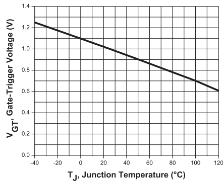
Typical Gate-Trigger Voltage
