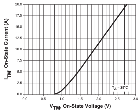
Typical On-State Voltage
